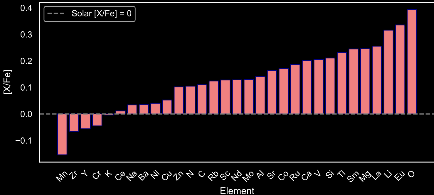
Abundance Pattern for GALAH Red Giants: Star Field [30] (N=35)
