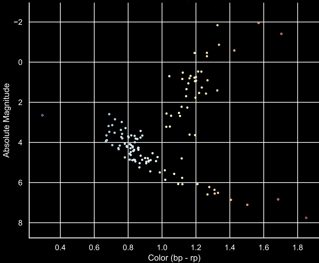
GALAH Hertzprung-Russel Diagram Field [30] Ra [322.36] Dec [-48.12]
