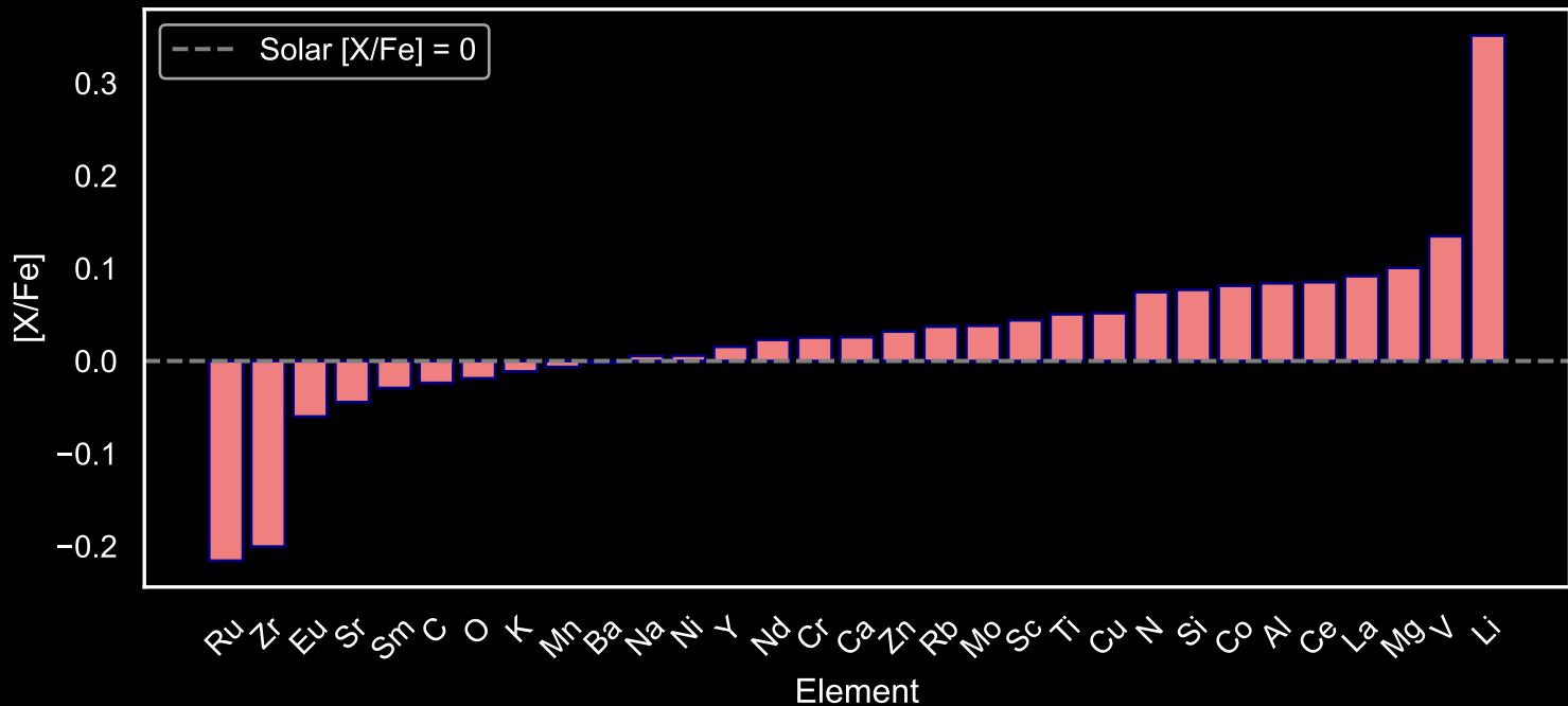
Abundance Pattern for GALAH Main Sequence Stars: Star Field [30] (N=63)
