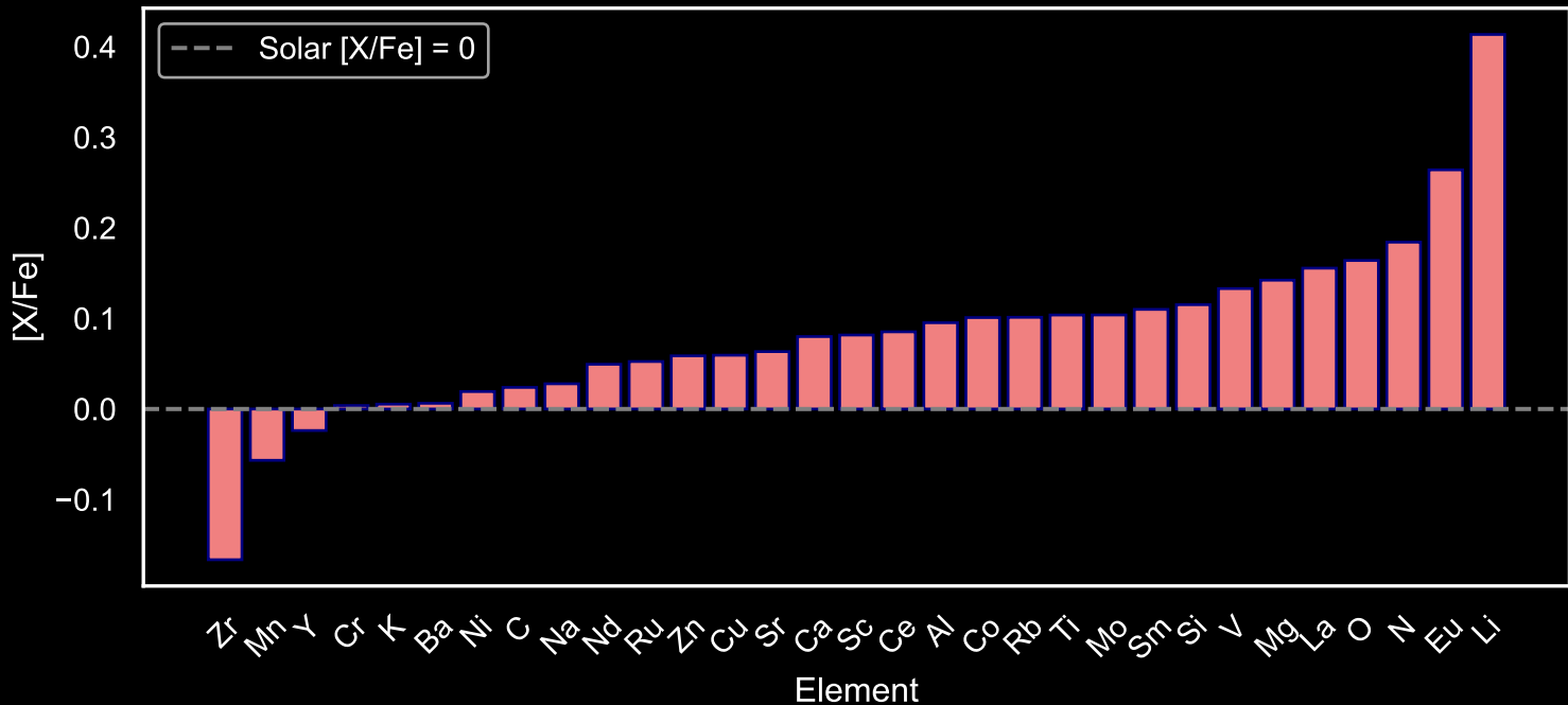
Abundance Pattern for GALAH Star Field [30] (N=128)
