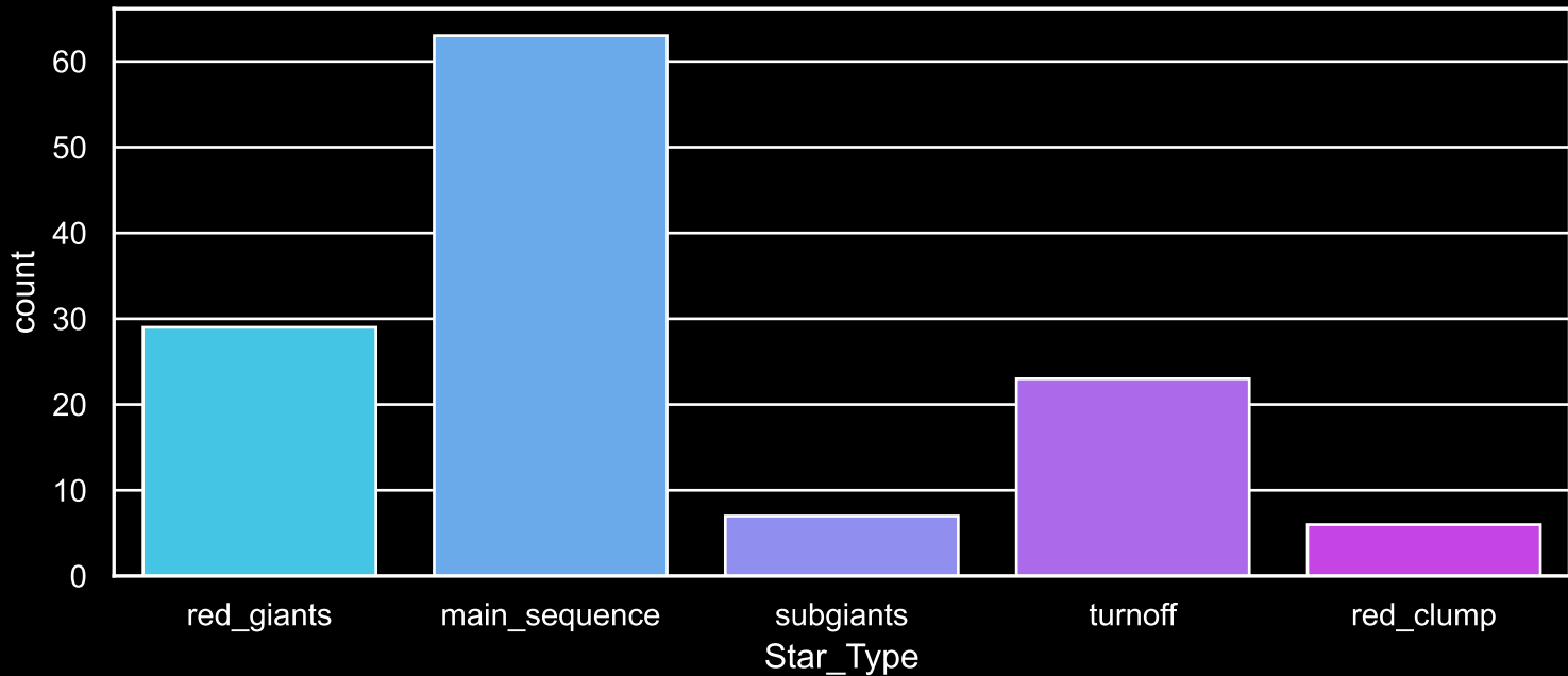
Field [30] Count plot of Star Type
